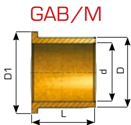
GAP-MET®/M Flange bushing
