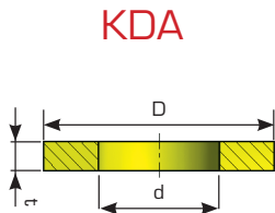
COM-KU®/D Thrust washer
