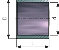
FER-MAN®259 Flange bushing
