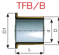
TEF-MET®/B Flange bushing
