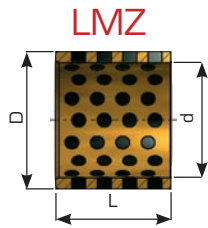
LUB-MET® Cylindrical bushing
