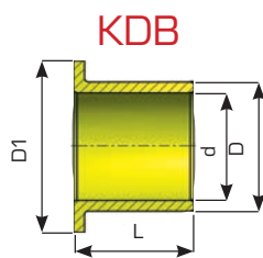
COM-KU®/D Flange bushing
