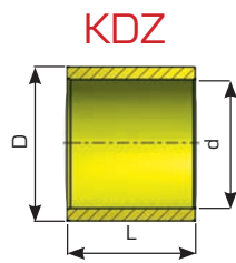
COM-KU®/D Cylindrical bushing
