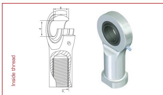
Rod end, steel / steel with inside thread
