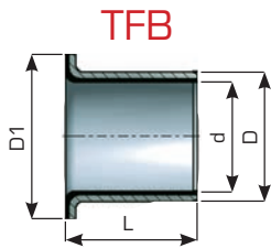
TEF-MET® Flange bushing
